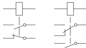
Auxiliary relay with mechanical contacts
