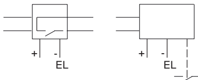
Static relay with terminals for external auxiliary voltage supply
