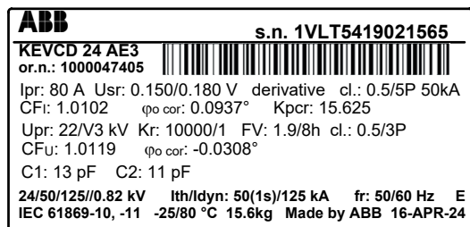
09 Example of a sensor label according to IEC 61869-10,-11
