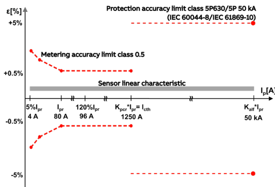
O5 Example of combined accuracy class for current measurement
