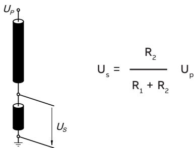
O3 Resistive divider principle
