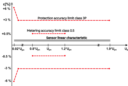
O6 Example of combined accuracy class for voltage measurement
