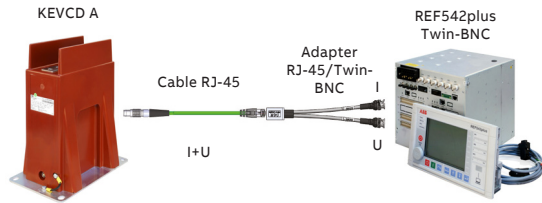
13 Connection between sensor and IED which requires adapter
