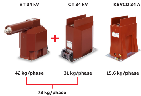
O7 Combined sensors
