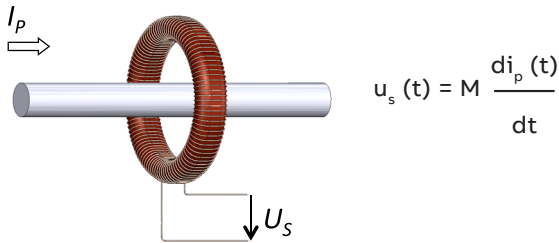
O2 Rogowski coil principle
