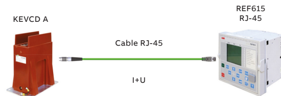
12 Direct connection between the sensor and IED
