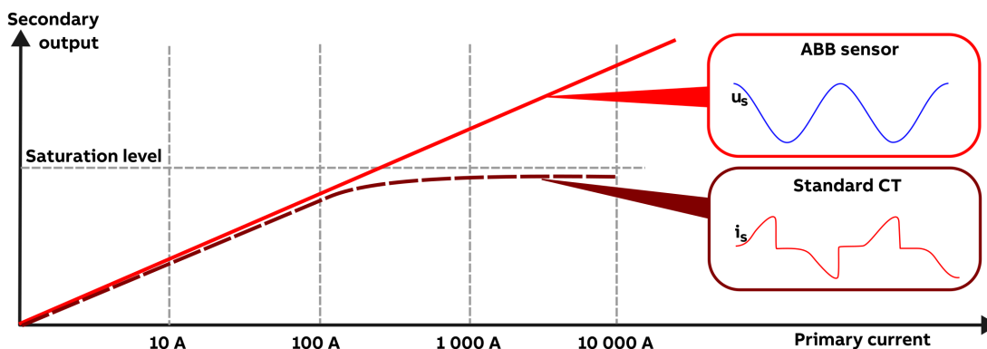
O1 Example of sensor characteristic and current characteristic
