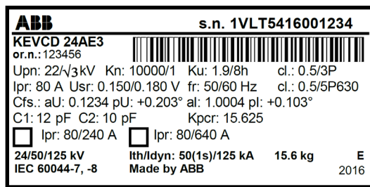
08 Example of a sensor label according to IEC 60044-7,-8
